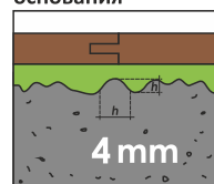
sub-floor levelling
